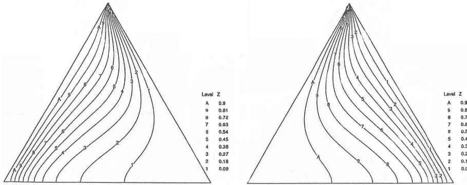
FIGURE 2. The mirror images of distortions of concentration field for gravity downward direction(left) and gravity upward direction(right) with L_e = 1 , B = 0 , R_a = 100 , and \beta = 0.33\pi .
