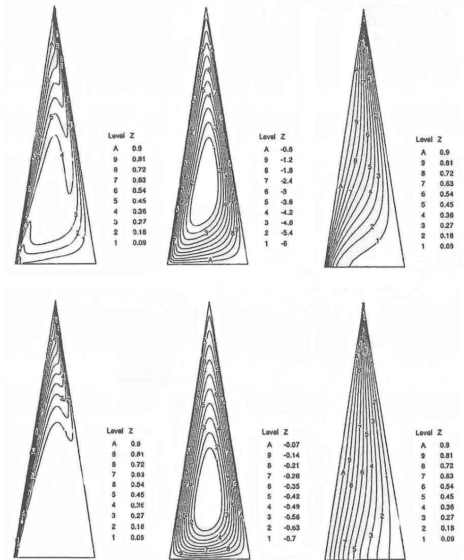
FIGURE 3. Steady state solution of concentration(left), flow(middle), and temperature(right) fields for L_e = 10 , B = 0 , and R_a = 100 case(top) and L_e = 100 , B = 0 , and R_a = 10 case(bottom)with gravity downward direction.
